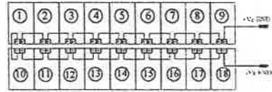
TYPICAL MODULE INTERCONNECTION DETAILS
